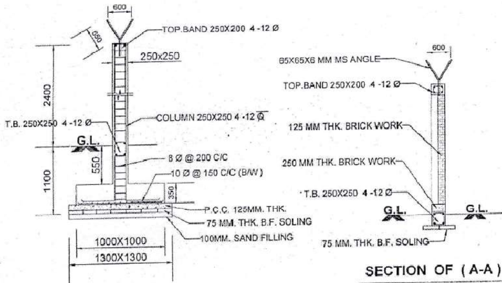
DETAILS OF R.C.C. FOUNDATION
