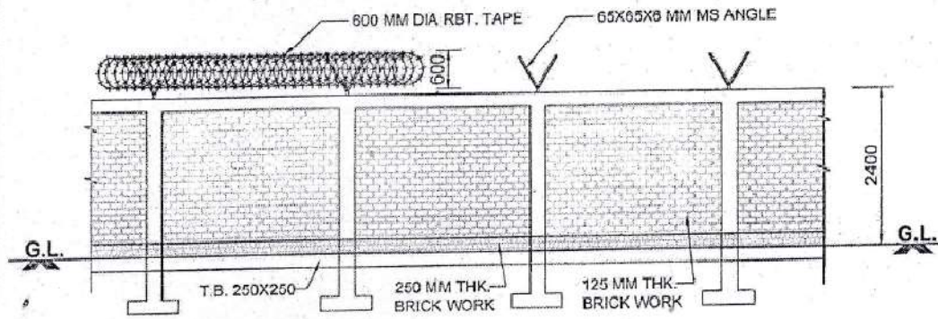
FRONT ELEVATION OF BOUNDARY
