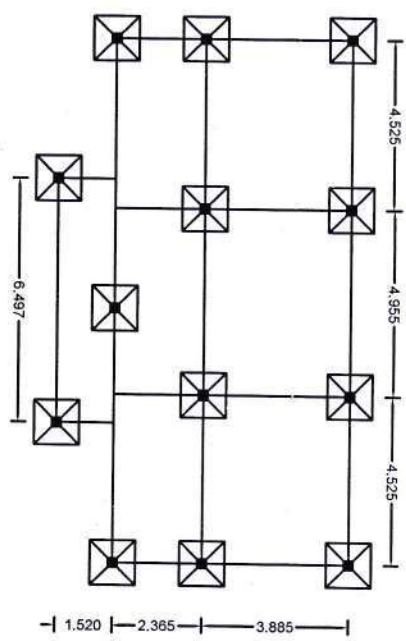
LAYOUT PLAN
