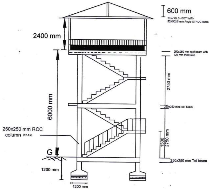
CROSS SECTIONAL ELEVATION
