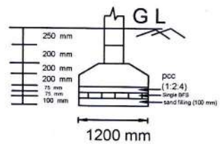
Foundation Details
