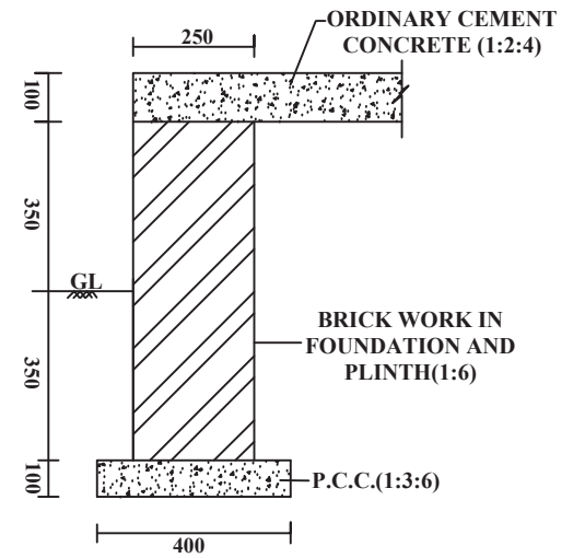
CROSS SECTION OF GUARD WALL
