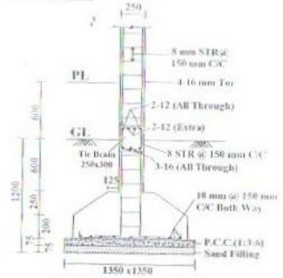
DETAILS OF R.C.C COLUMN FOUNDATION
