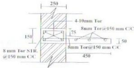
DETAILS OF R.C.C LINTEL AND CHAJJA
