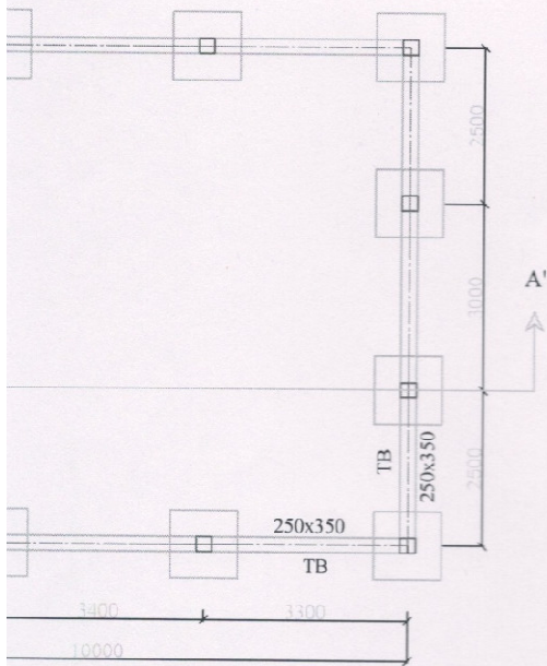
FOUNDATION LAYOUT OF LIZARD ENCLOSURE
