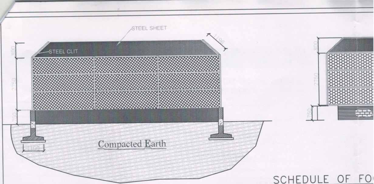
A-A' SECTION ELEVATION OF LIZARD ENCLOSURE
