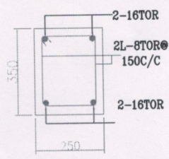
TYP. SEC OF TIE BEAM (TB) SCALE 1:30
