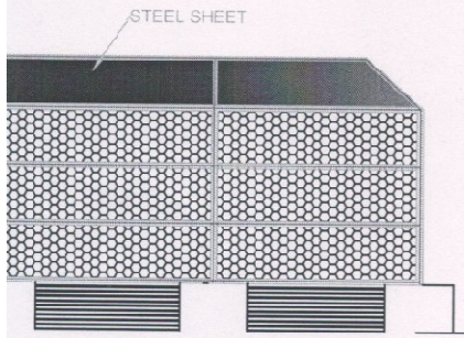
FRONT ELEVATION OF LIZARD ENCLOSURE
